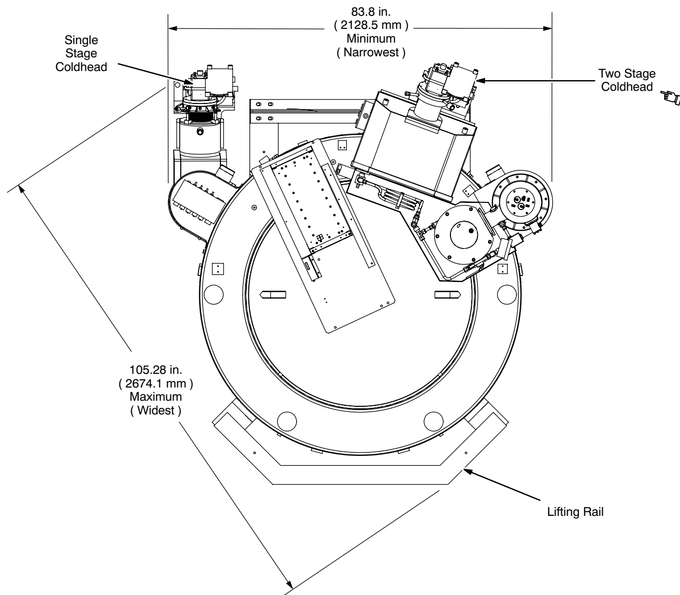
MINUMUM / MAXIMUM MAGNET DIMENSIONS ILLUSTRATION 6-2
