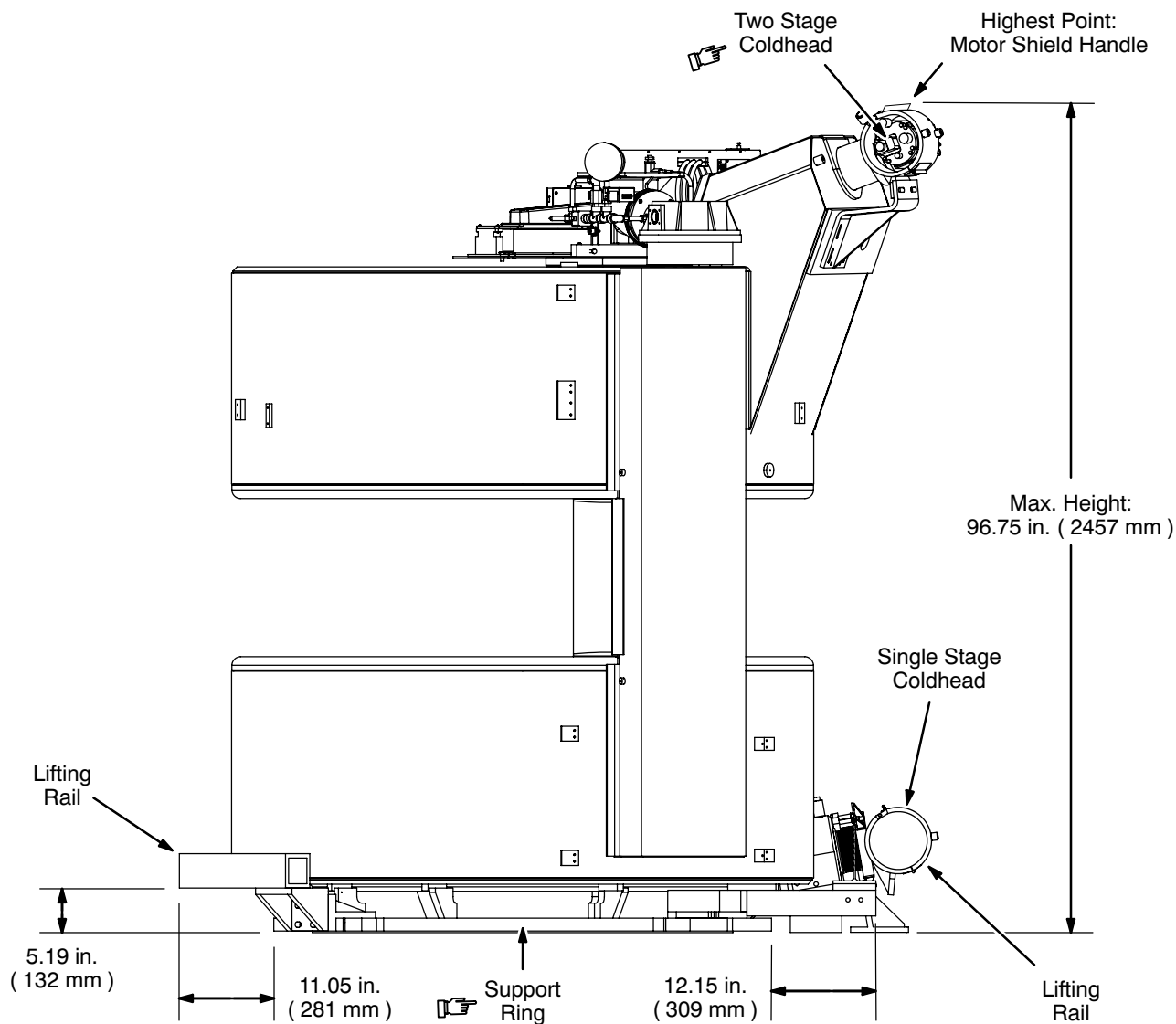
MAGNET CLEARANCES ILLUSTRATION 6-1
